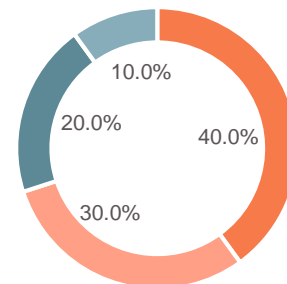
Target
